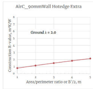
AirC_Cleva Pod® 90mmWall Hotedge Extra
