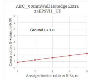
AirC_Cleva Pod® 90mmWall Hotedge Extra 25EPSVH_UF
